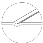
V MODEL
