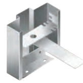
"T" masonry anchor (TMA) shipped loose. Includes floor anchors
